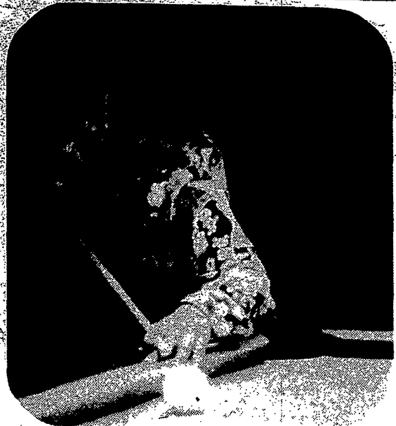
Taking aim during a recreation period.
